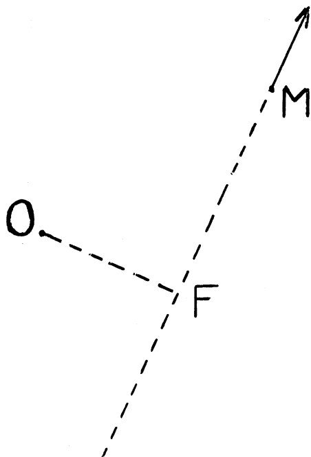
FIG. 1. Angular momentum. M is a material point, O a geometric reference point. The vector arrow represents the momentum (= mass times velocity) of M. Then the angular momentum is the product of the length of the arrow by the length OF.
